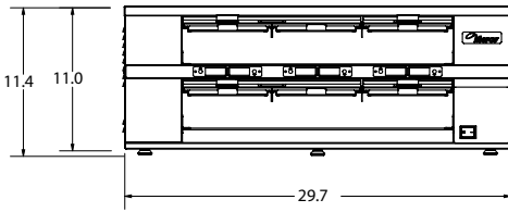
MHG42 with timer bars
