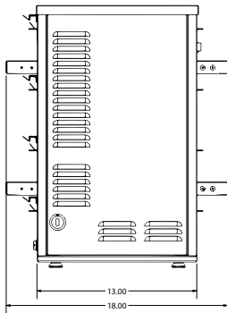
MHG42 with timer bars
