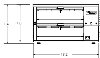
MHG22 without timers
