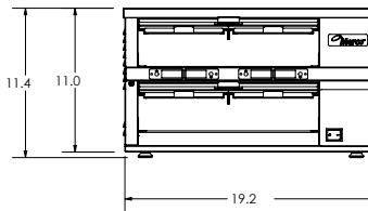
MHG34 with timer bars MHG32 with timer bars
