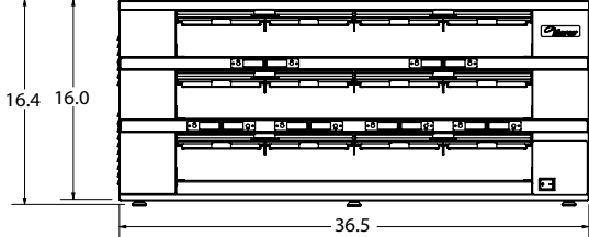
MHG22 without timers
